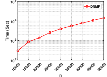
Fig. 7: Scalability testing.
