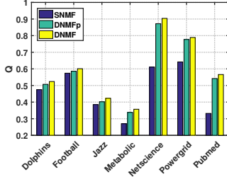
Fig. 5: Ablation study.
