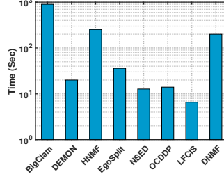
Fig. 6: Running time comparison.
